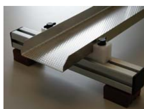
TRAY MOUNTING AT EXIT END WITH GUIDE BLOCKS
